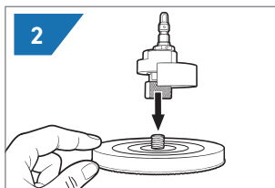
2. SCREW THE BACKING PAD INTO THE SPINDLE IN A CLOCK-WISE DIRECTION. HAND TIGHTEN ONLY.
