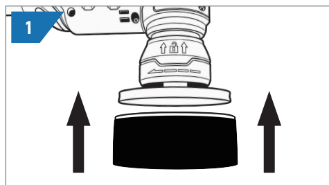
1. TO FIT, PUSH THE FOAM PAD ONTO THE HOOK & LOOP BACKING PAD.
