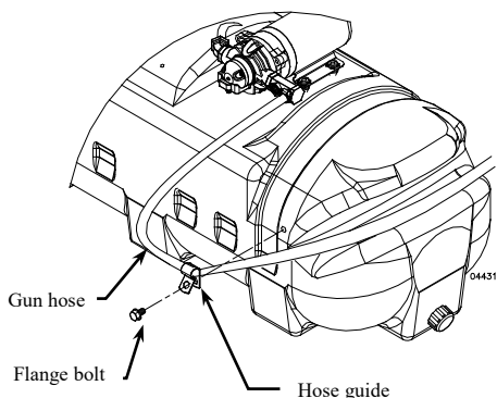
Hose guide
