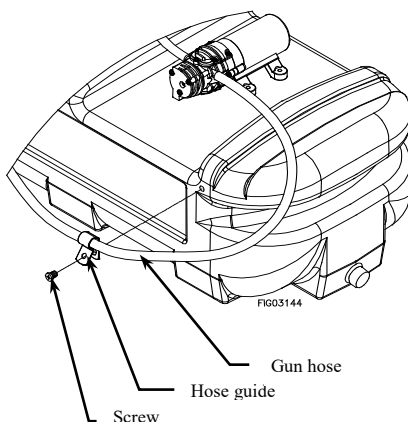
Screw
