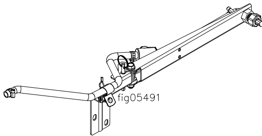
Right Broadcast Boom Assembly (Qty 1)
