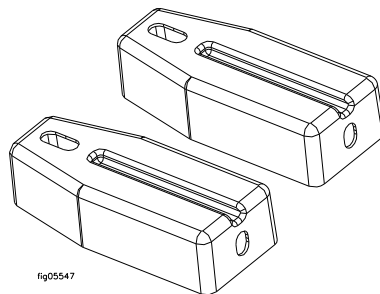
K16004-51 Front Tank Bracket Qty 2
