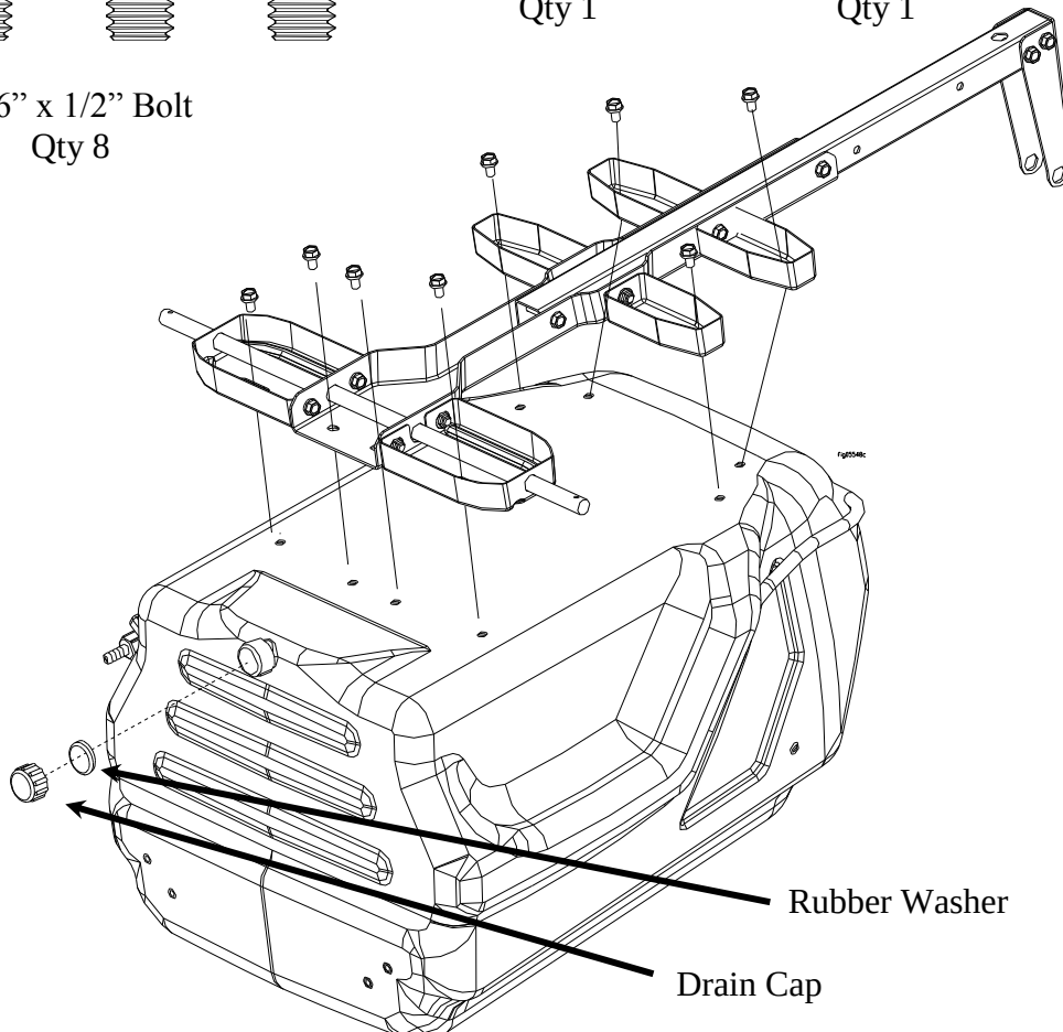
K16003-2 Rubber Washer Qty 1
