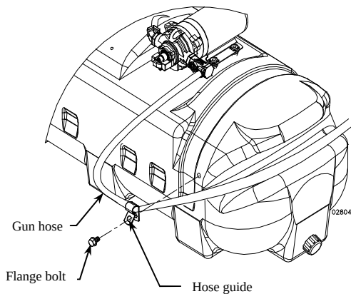
Hose guide
